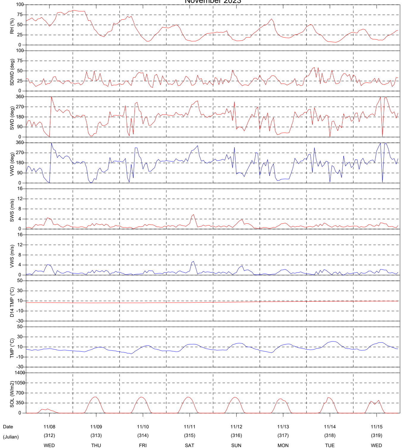
Figure 4-8 Colorado Air Toxics - B1 (DuPont Elementary School) - Hourly Meteorological Data November 2023
