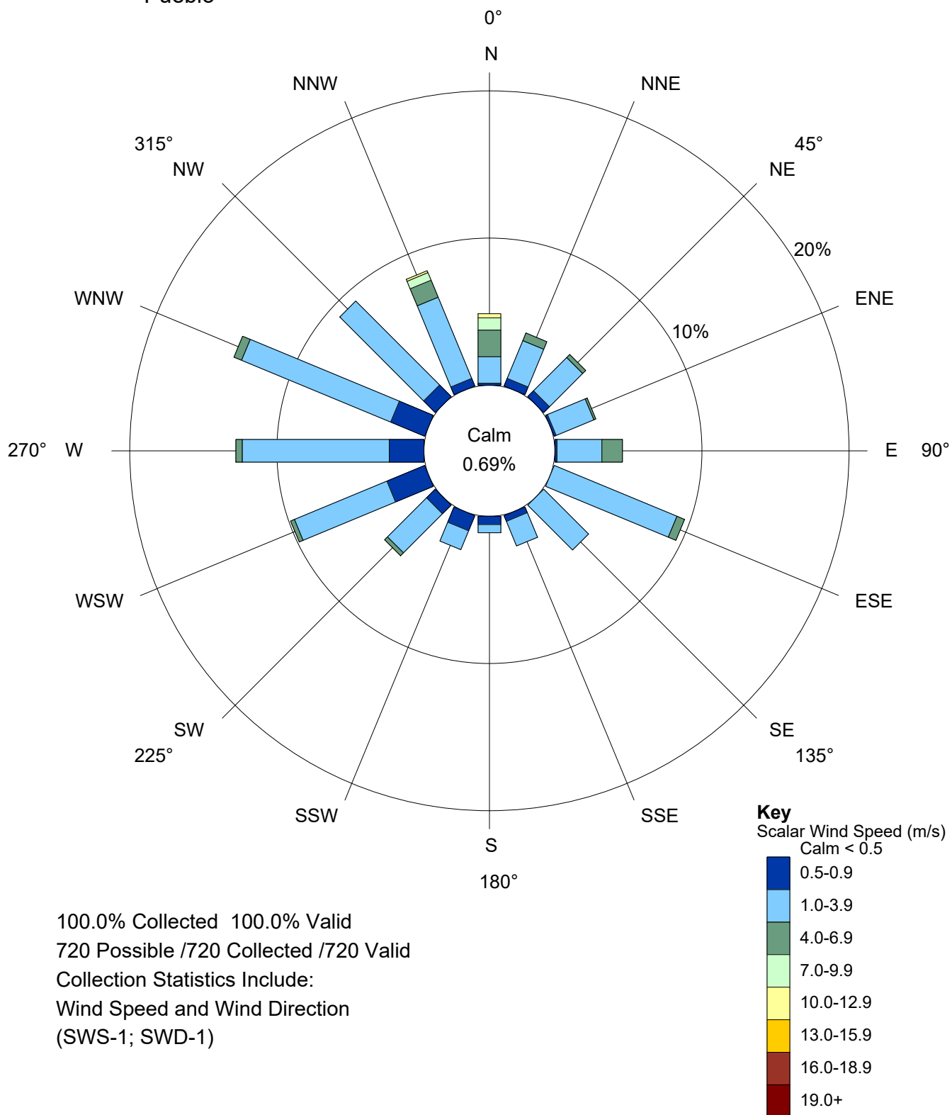
Figure 4-11 Colorado Air Toxics - C1 Pueblo Wind Rose 11/01/2023 - 11/30/2023
