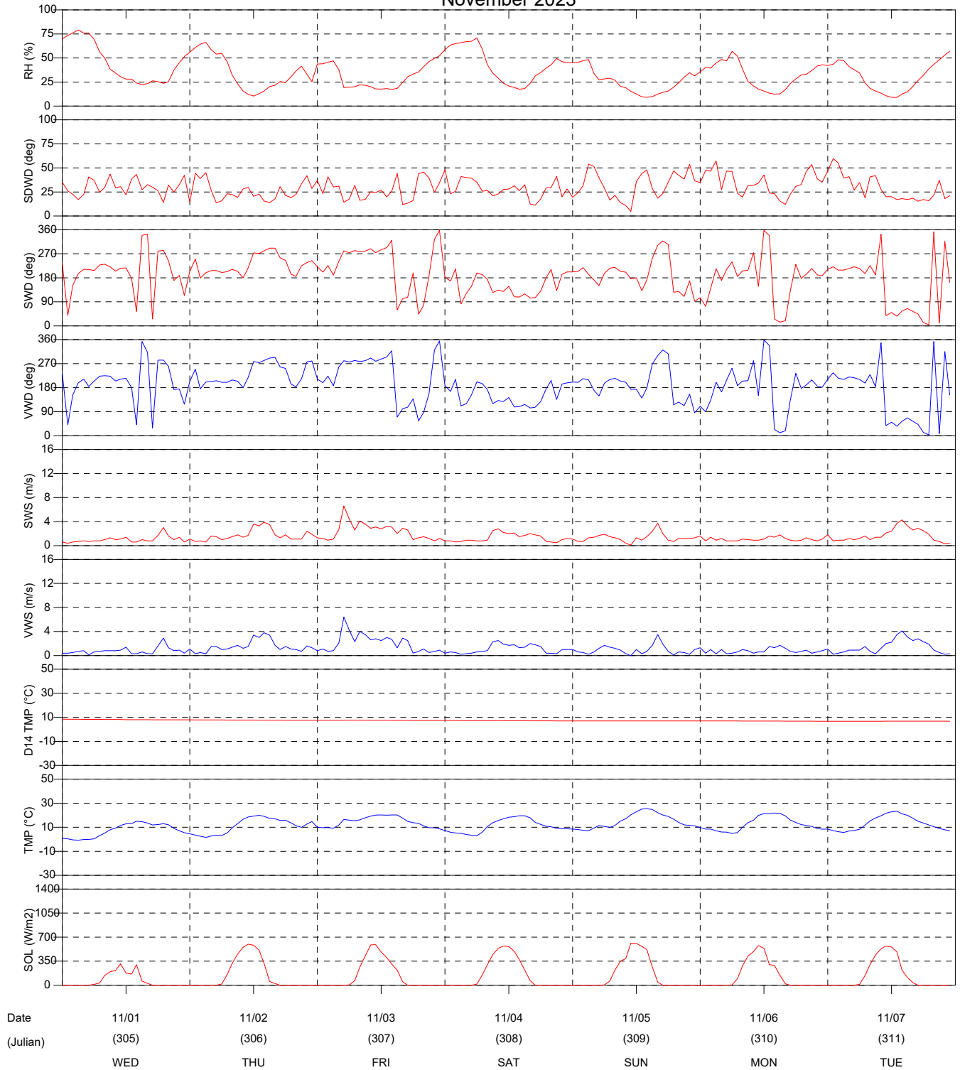
Figure 4-7 Colorado Air Toxics - B1 (DuPont Elementary School) - Hourly Meteorological Data November 2023
